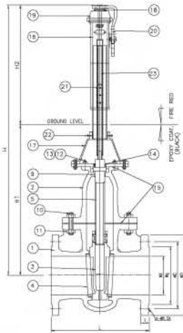
(POST INDICATOR GATE VALVE)
